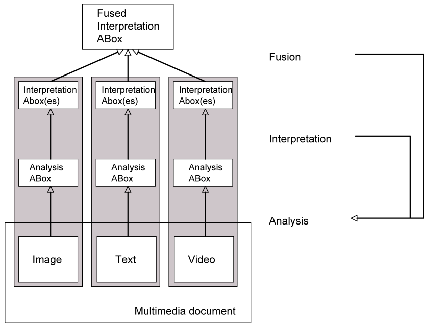
Figure 26: Multimedia interpretation architecture.
