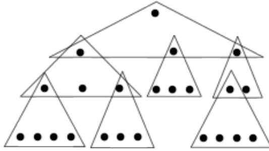
Figure 29: Structure of aggregate hierarchy induced by aggregate structure. The quasi-tree structure reflects abstraction properties and allows for efficient probabilistic inferences.
