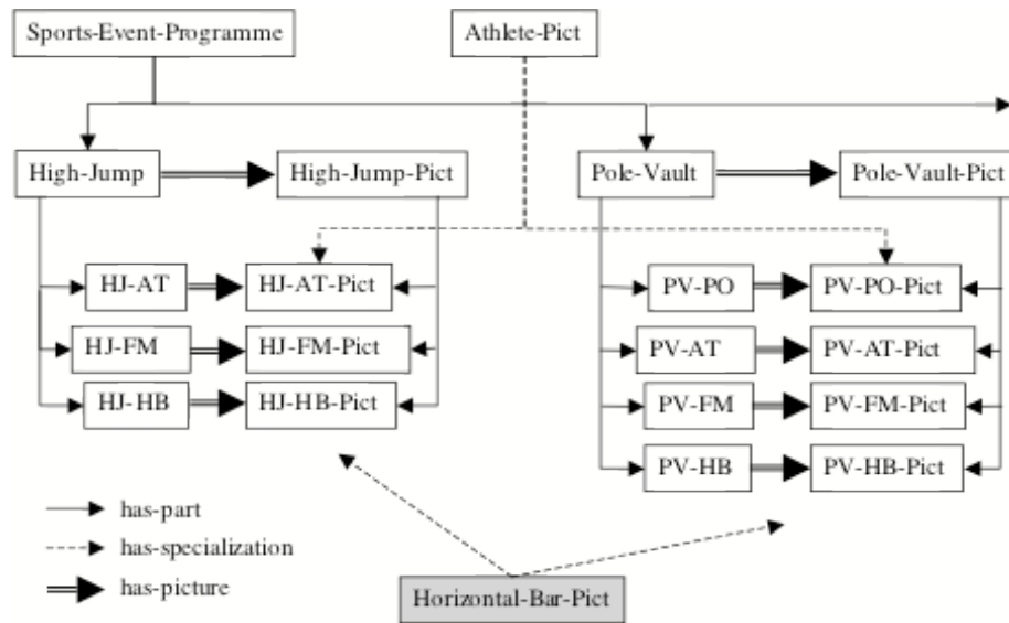
Figure 27: Aggregate concepts relating a high jump and a pole vault to corresponding media object concepts. The Horizontal-Bar-Pict can be interpreted as an instance of a high-jump-horizontal-bar picture ( HJ-HB-Pict ) or of a pole-vault-horizontal-bar picture ( PV-HB-Pict ).
