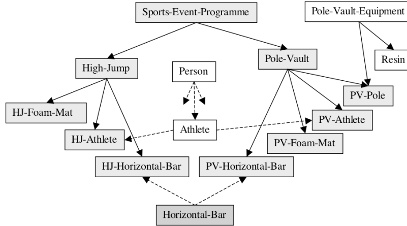
Figure 21: Compositional hierarchy induced by hasPart roles in aggregate concepts. The dotted arrows indicate specialisation relations.
