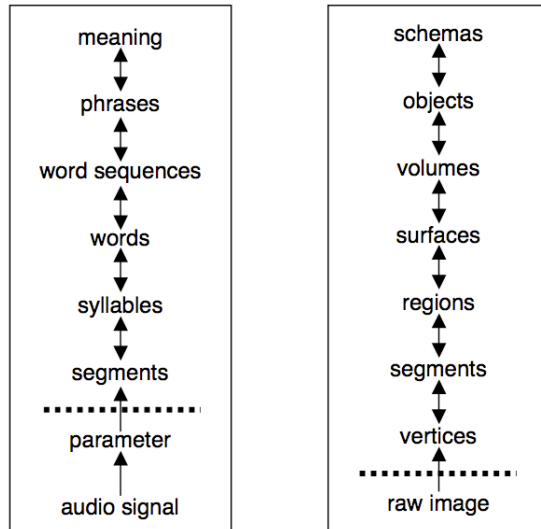
Figure 2: Typical level structure of media interpretation systems exemplified by HEARSAY II and VISIONS. Signal processing (below dotted line) transforms the raw input signals into primitive media objects, various interpretation processes lead up to higher-level interpretations.
